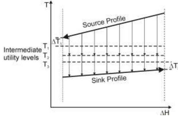
Figure 2: Selection of temperature of intermediate utility (developed after Ahmad et al., 1990)
